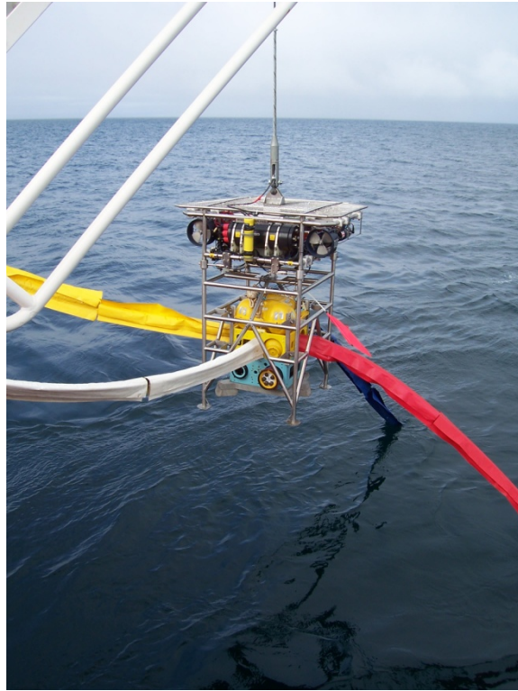
HyBIS Robotic Underwater Vehicle with NOC's OBS/OBEM Deployment Module
